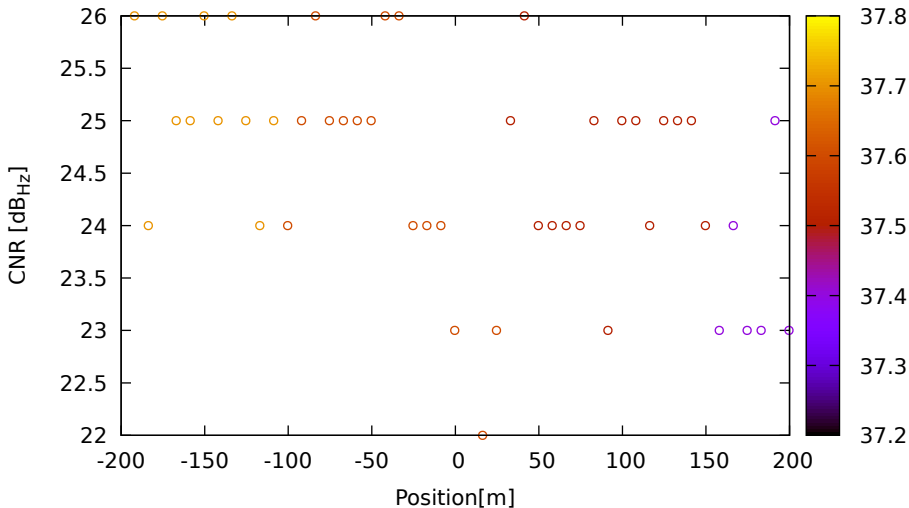
CNR vs position for E36 (E1) on HuaweiP40 - DOY 262 jam. 3
