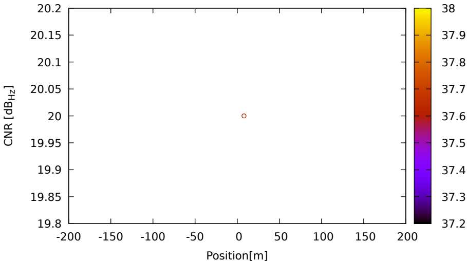
CNR vs position for E36 (E5a) on HuaweiP40 - DOY 262 jam. 3
