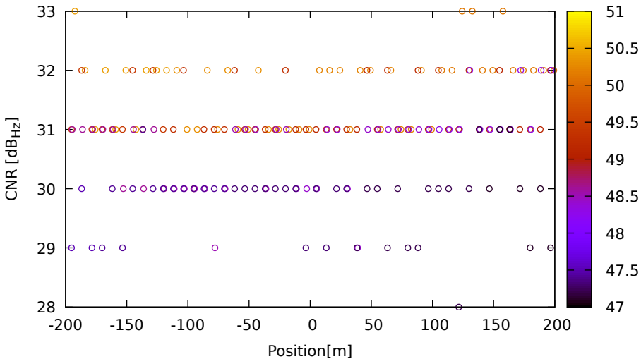
CNR vs position for G01 (L5) on HuaweiP40 - DOY 262 jam. 2
