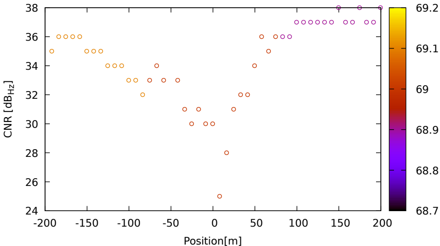
CNR vs position for G03 (G1) on HuaweiP40 - DOY 262 jam. 3
