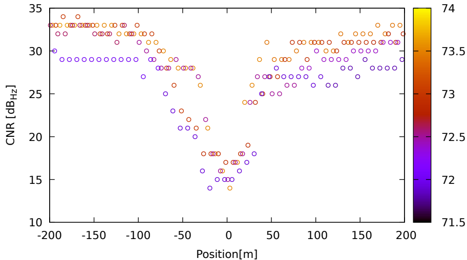
CNR vs position for G03 (L5) on HuaweiP40 - DOY 262 jam. 1
