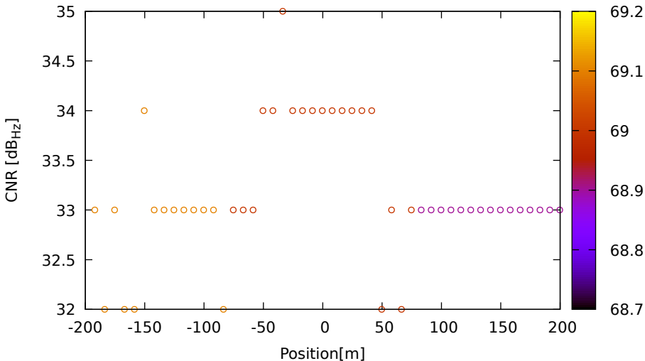
CNR vs position for G03 (L5) on HuaweiP40 - DOY 262 jam. 3
