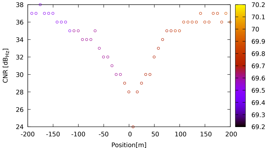
CNR vs position for G04 (G1) on HuaweiP40 - DOY 262 jam. 3
