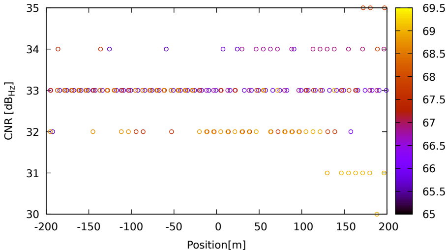
CNR vs position for G04 (L5) on HuaweiP40 - DOY 262 jam. 2
