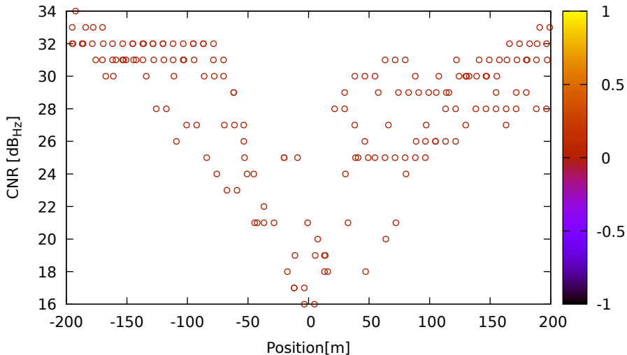
CNR vs position for G06 (L1) on HuaweiP40 - DOY 262 jam. 2
