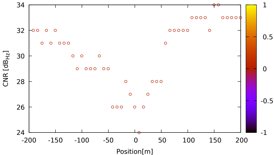
CNR vs position for G06 (L1) on HuaweiP40 - DOY 262 jam. 3
