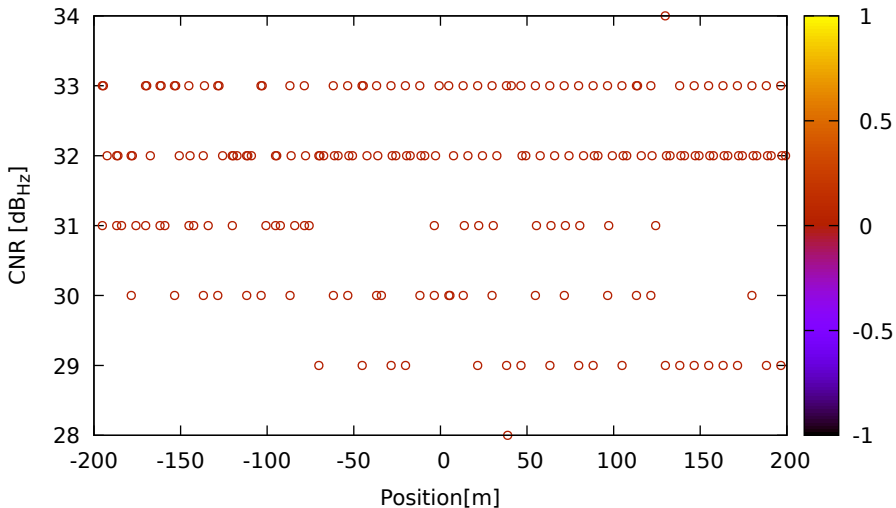
CNR vs position for G06 (L5) on HuaweiP40 - DOY 262 jam. 2
