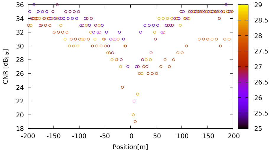
CNR vs position for G09 (G1) on HuaweiP40 - DOY 262 jam. 1
