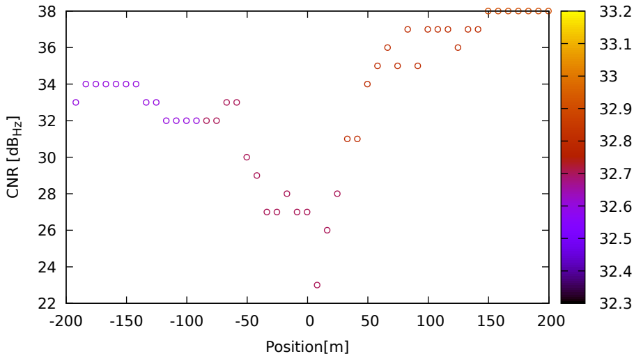
CNR vs position for G09 (G1) on HuaweiP40 - DOY 262 jam. 3
