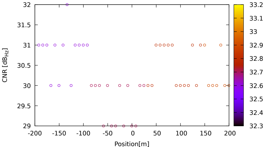
CNR vs position for G09 (L5) on HuaweiP40 - DOY 262 jam. 3
