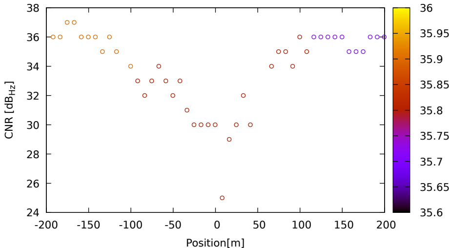
CNR vs position for G17 (G1) on HuaweiP40 - DOY 262 jam. 3
