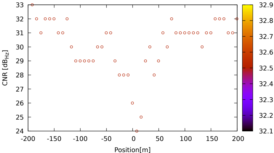
CNR vs position for G19 (G1) on HuaweiP40 - DOY 262 jam. 3
