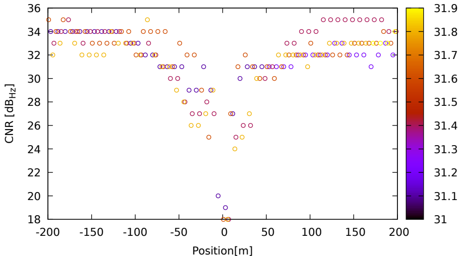
CNR vs position for G19 (L1) on HuaweiP40 - DOY 262 jam. 1
