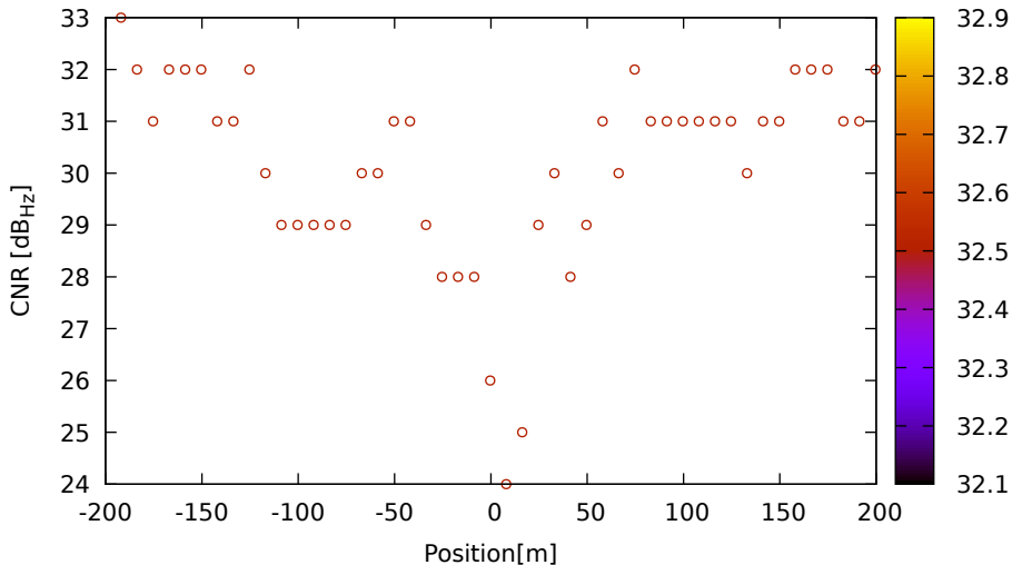
CNR vs position for G19 (L1) on HuaweiP40 - DOY 262 jam. 3
