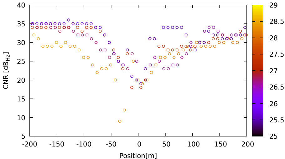
CNR vs position for G21 (G1) on HuaweiP40 - DOY 262 jam. 2
