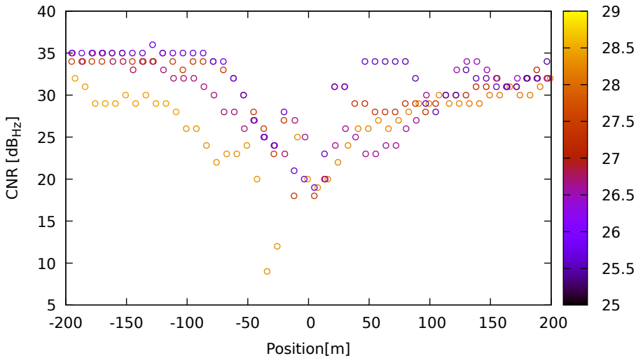
CNR vs position for G21 (L1) on HuaweiP40 - DOY 262 jam. 2
