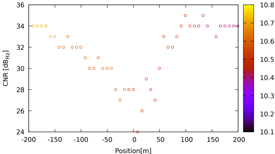
CNR vs position for G22 (G1) on HuaweiP40 - DOY 262 jam. 3
