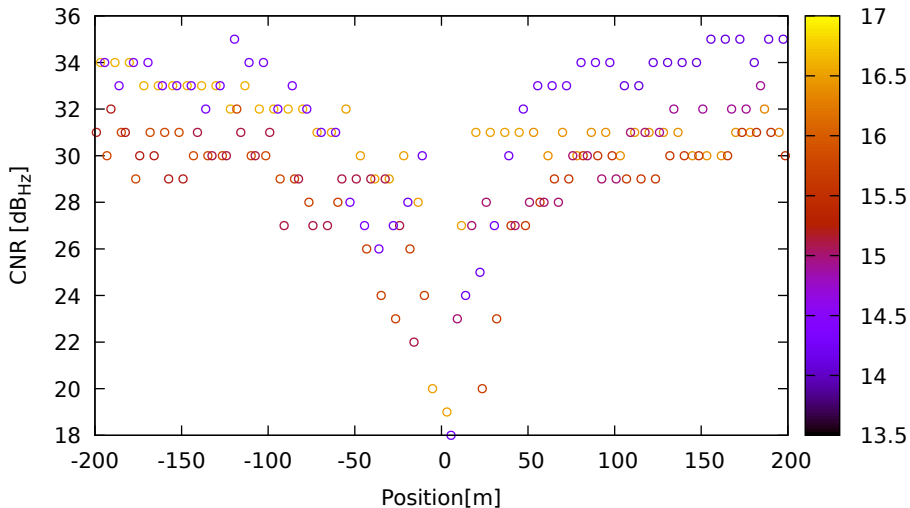
CNR vs position for G22 (L1) on HuaweiP40 - DOY 262 jam. 1
