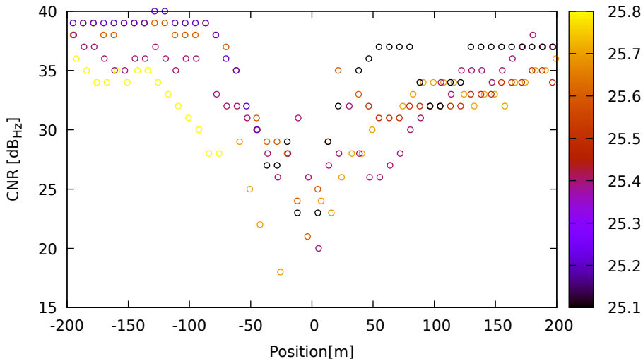
CNR vs position for G31 (G1) on HuaweiP40 - DOY 262 jam. 2
