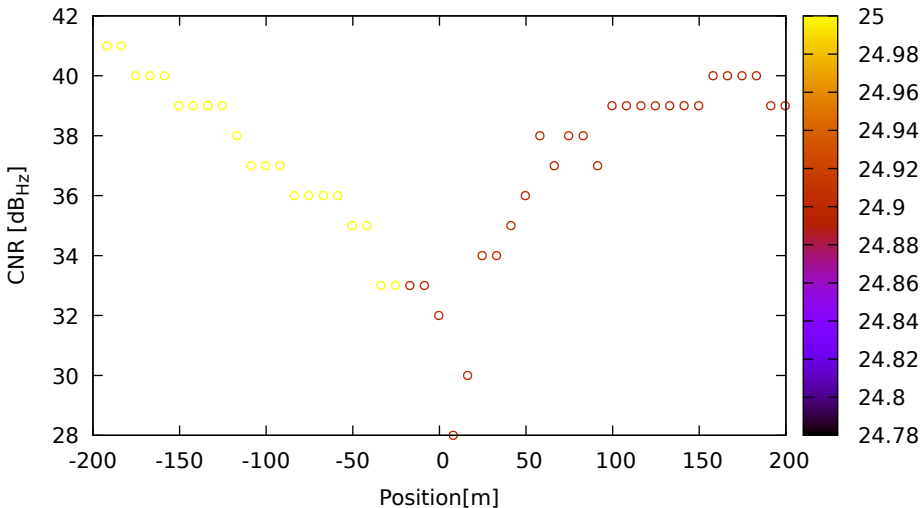
CNR vs position for G31 (G1) on HuaweiP40 - DOY 262 jam. 3
