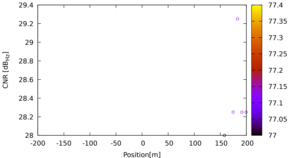
CNR vs position for E05 (E5a) on Xiaomi11T - DOY 262 jam. 1
