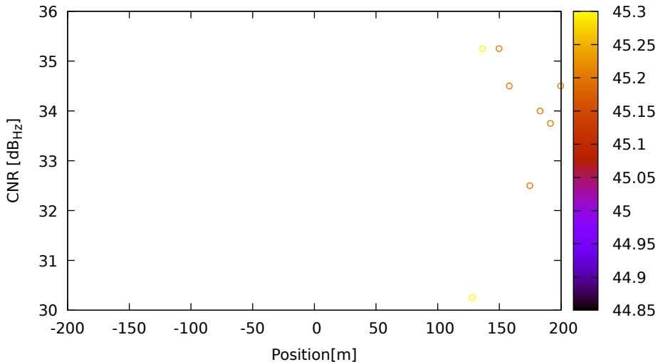
CNR vs position for E09 (E5a) on Xiaomi11T - DOY 262 jam. 1
