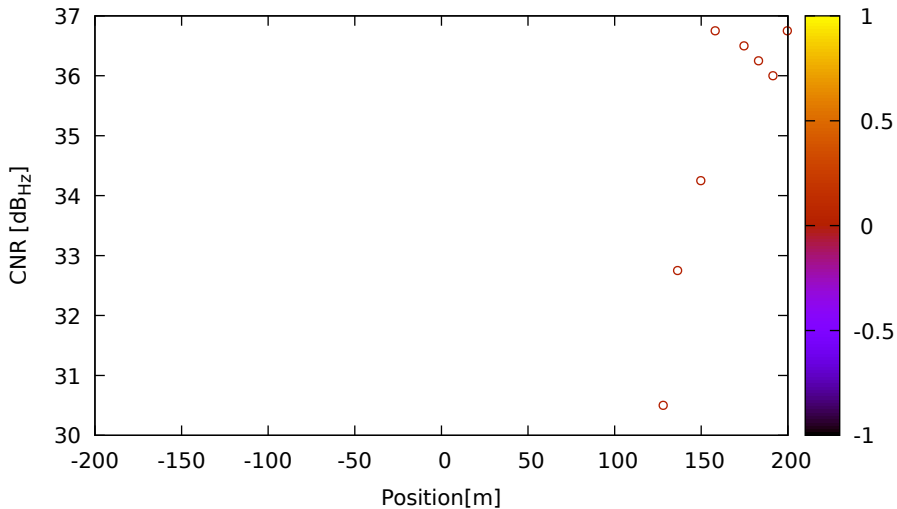
CNR vs position for E14 (E5a) on Xiaomi11T - DOY 262 jam. 1
