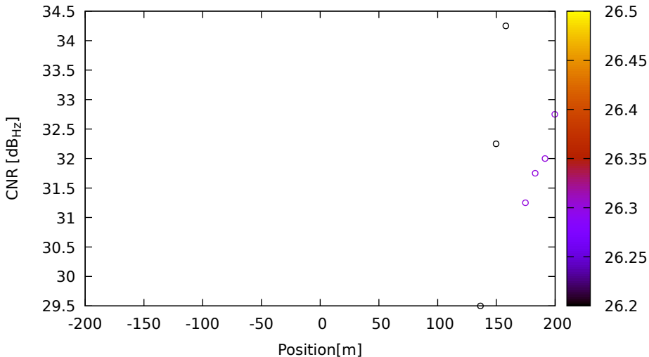
CNR vs position for E15 (E5a) on Xiaomi11T - DOY 262 jam. 1
