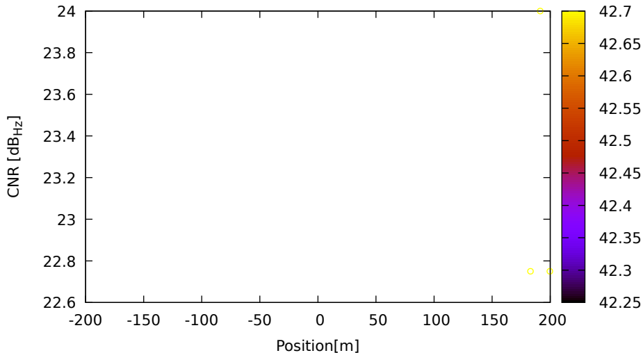
CNR vs position for E36 (E5a) on Xiaomi11T - DOY 262 jam. 1
