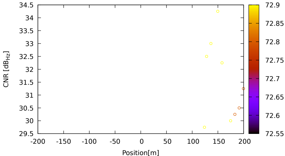
CNR vs position for G03 (L5) on Xiaomi11T - DOY 262 jam. 1
