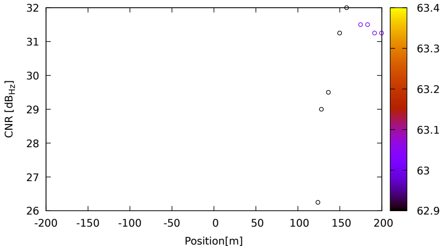
CNR vs position for G04 (L5) on Xiaomi11T - DOY 262 jam. 1
