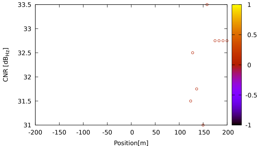
CNR vs position for G06 (L5) on Xiaomi11T - DOY 262 jam. 1
