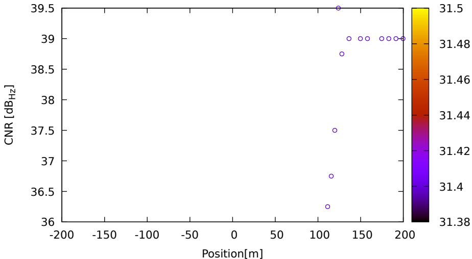
CNR vs position for G19 (L1) on Xiaomi11T - DOY 262 jam. 1
