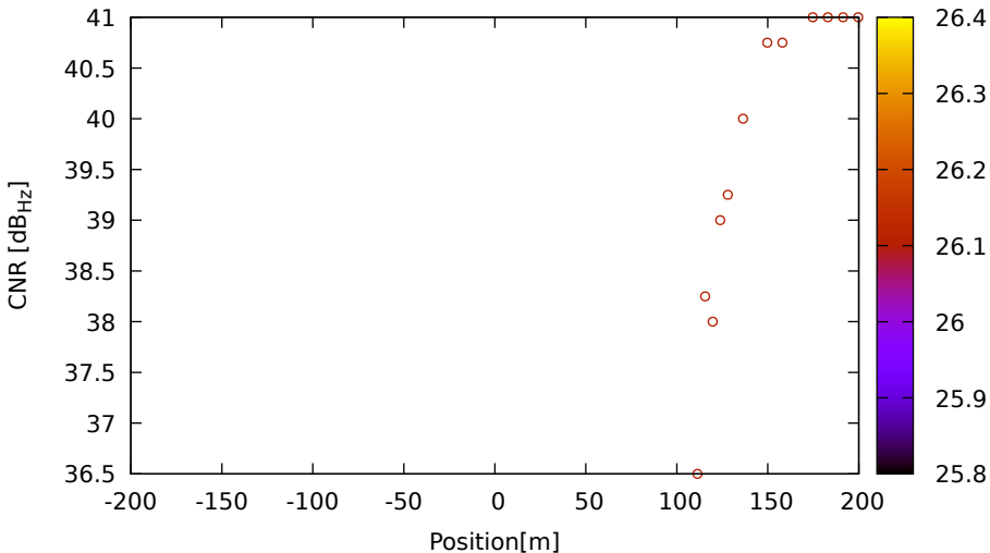
CNR vs position for G31 (L1) on Xiaomi11T - DOY 262 jam. 1
