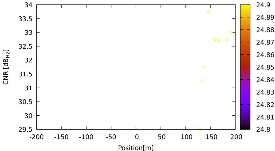
CNR vs position for C06 (B1) on XiaomiMi8 - DOY 262 jam. 1
