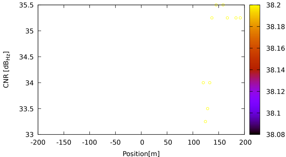
CNR vs position for C09 (B1) on XiaomiMi8 - DOY 262 jam. 1
