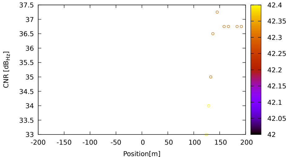
CNR vs position for C14 (B1) on XiaomiMi8 - DOY 262 jam. 1
