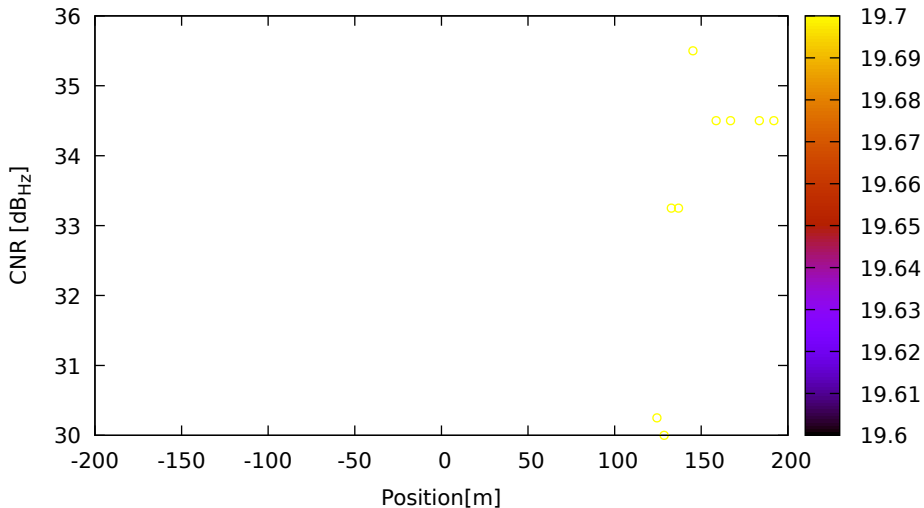
CNR vs position for C16 (B1) on XiaomiMi8 - DOY 262 jam. 1
