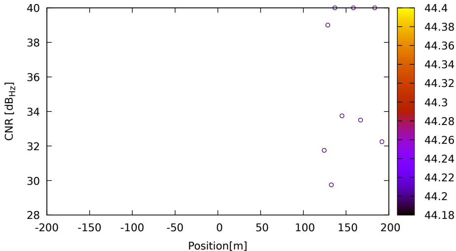
CNR vs position for C27 (B1) on XiaomiMi8 - DOY 262 jam. 1
