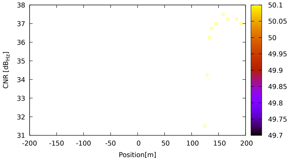
CNR vs position for C28 (B1) on XiaomiMi8 - DOY 262 jam. 1
