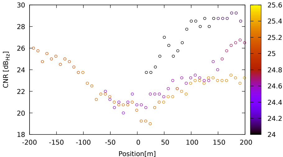
CNR vs position for E03 (E5a) on XiaomiMi8 - DOY 262 jam. 1
