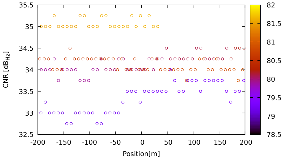
CNR vs position for E05 (E5a) on XiaomiMi8 - DOY 262 jam. 2
