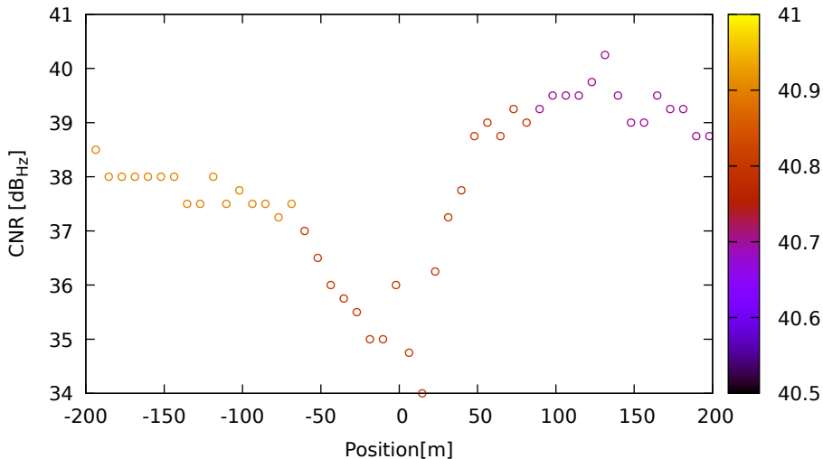
CNR vs position for E09 (E1) on XiaomiMi8 - DOY 262 jam. 3
