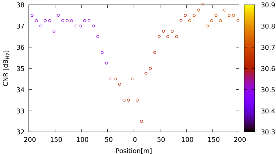
CNR vs position for E15 (E1) on XiaomiMi8 - DOY 262 jam. 3
