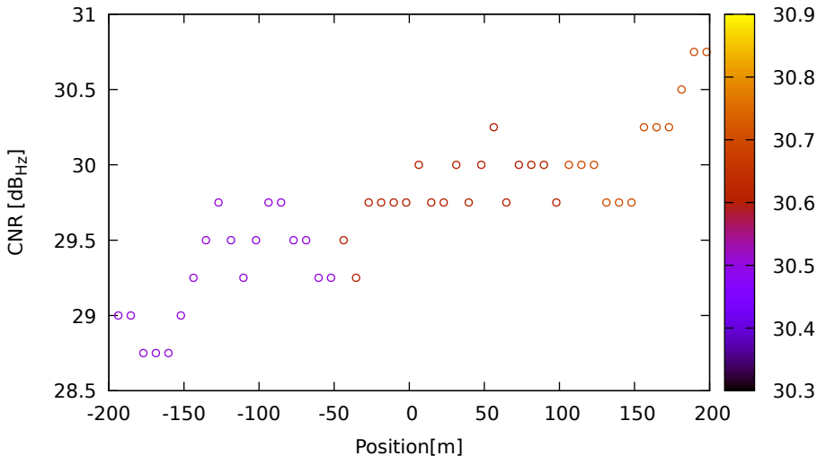
CNR vs position for E15 (E5a) on XiaomiMi8 - DOY 262 jam. 3
