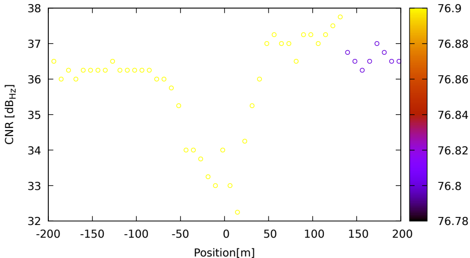
CNR vs position for E34 (E1) on XiaomiMi8 - DOY 262 jam. 3
