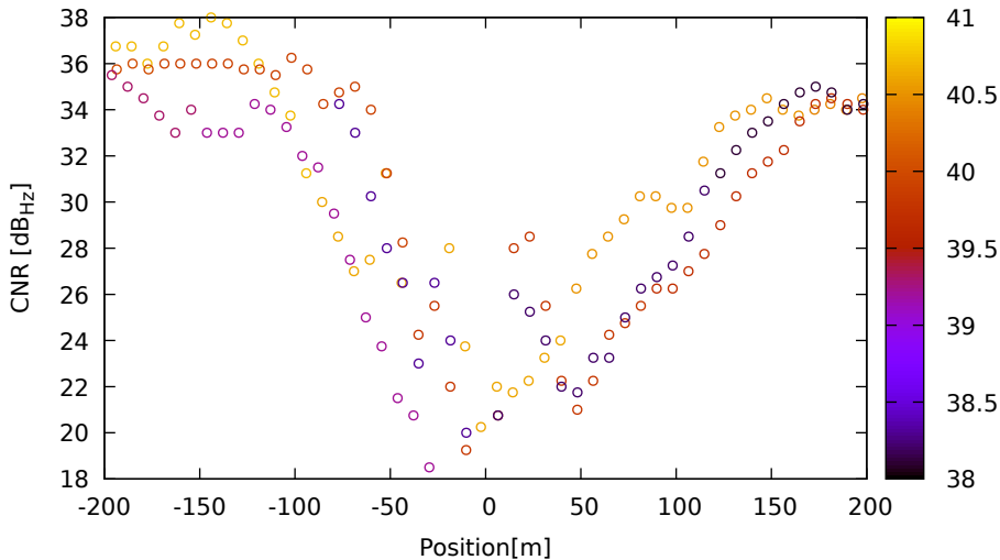
CNR vs position for E36 (E1) on XiaomiMi8 - DOY 262 jam. 2
