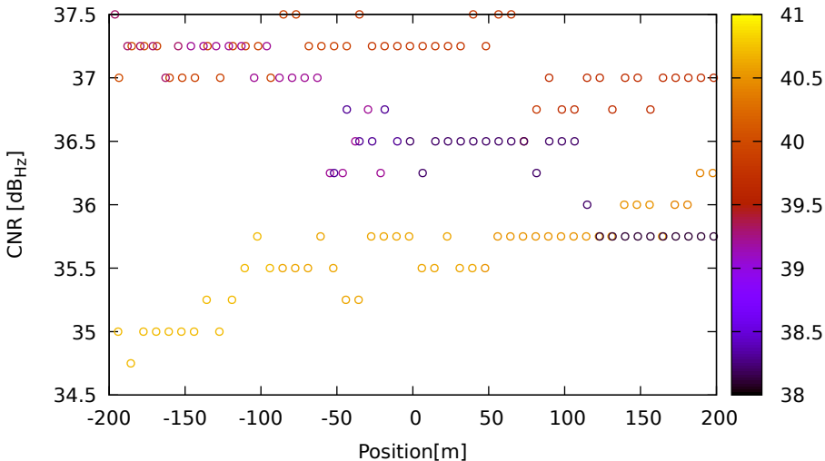
CNR vs position for E36 (E5a) on XiaomiMi8 - DOY 262 jam. 2
