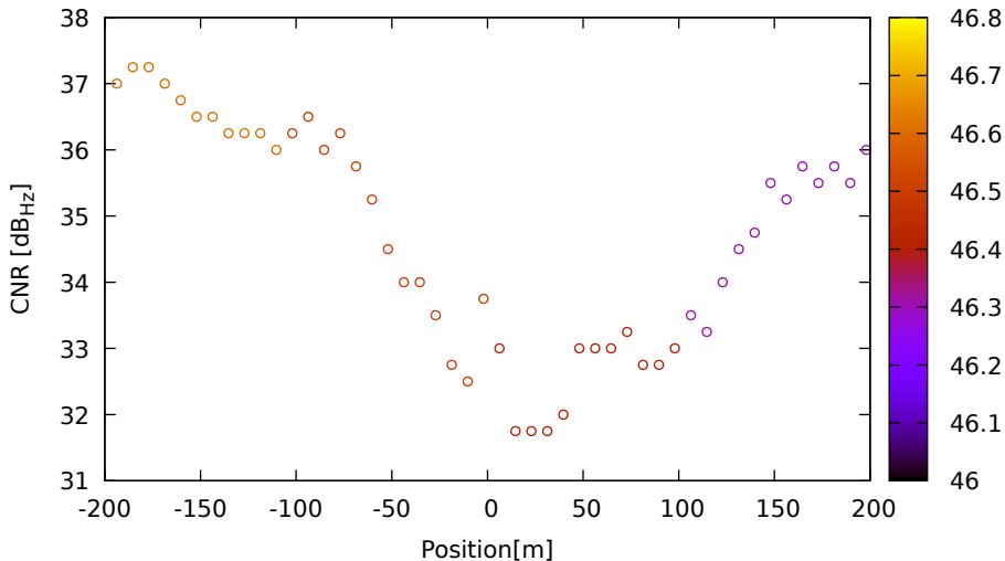
CNR vs position for G01 (L1) on XiaomiMi8 - DOY 262 jam. 3
