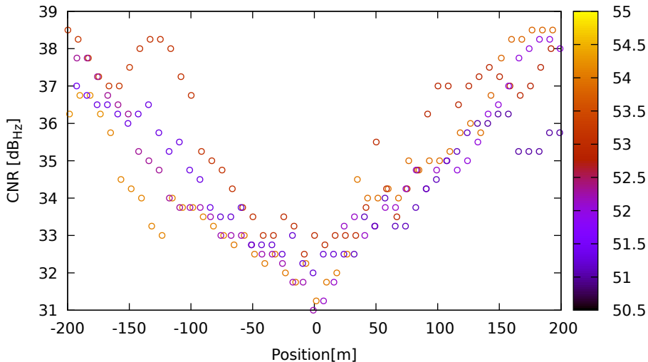
CNR vs position for G01 (L5) on XiaomiMi8 - DOY 262 jam. 1
